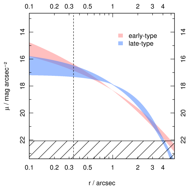
Figure 23. Surface brightness variation from u through to K for the early-type spheroid-dominated and late-type disk-dominated populations. We generate Sérsic indices and half-light radii in wavelength steps from u \rightarrow K for each population using the trends as described in equations 10, 11, 14 and 15. Using these values, surface brightness profiles (without PSF convolution) may be constructed for each wavelength bin. The shaded regions shown here represent the maximal area swept out by these light profiles along the transition from u through to K , and represent how much of an effect the reported changes in Sérsic index and half-light radius have on the overall light profiles. The hatched region indicates the brightest limit at which light profiles may be trusted ( \mu_{\text{lim},K} = 22.07 \text{ mag/arcsec}^{-2} ), and the vertical dashed line represents 1 pixel in distance from the centre. Profiles are produced assuming a constant total magnitude of m_{\text{tot}} = 15 for both the spheroid and disk populations.
