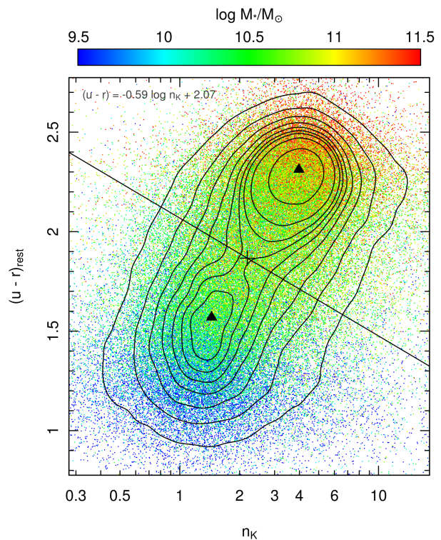
Figure 20. K band Sérsic index versus u - r rest frame colour, with the data points coloured according to their galaxy stellar mass estimates, as shown. Contours range from the 10^{\text{th}} to the 90^{\text{th}} percentile in steps of 10%. The two highest peaks in object density, corresponding to two distinct galaxy populations (late-type and early-type for low-index and high-index respectively), are represented by filled black triangles. The diagonal line lies perpendicular to the line connecting these two peaks, and bisects it at the point of lowest object density along the connecting line, marked on the figure with a plus sign. This dividing line defines two sub-samples, which for the most massive galaxies, relate to disk-dominated systems below the line (LTGs) and spheroid-dominated systems above (ETGs), the equation of which is inset into the Figure.
