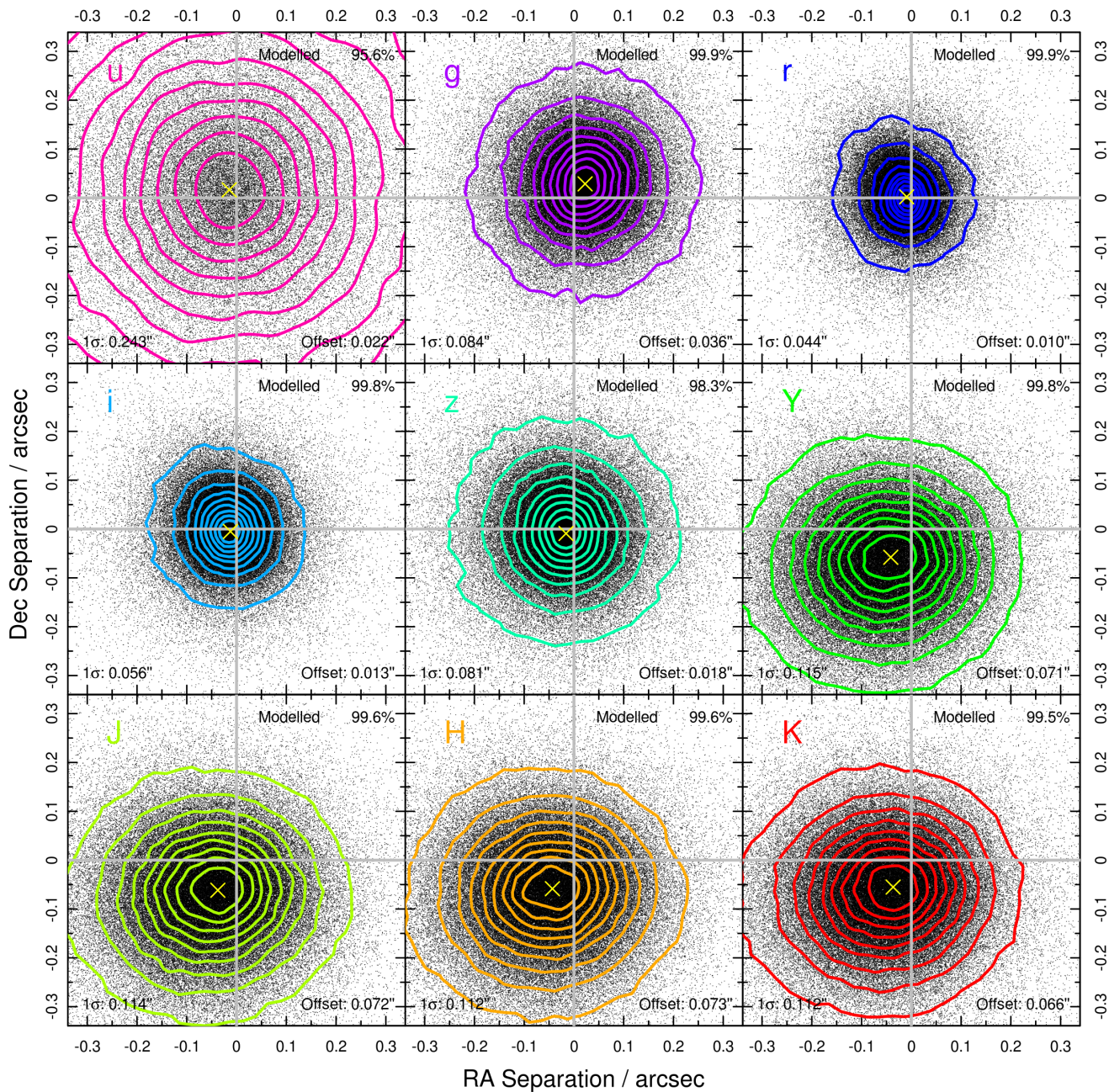
Figure 9. Astrometric offsets in RA and Dec between the input SDSS positions and the modelled SIGMA positions for all nine bands. Contours range from the 10 th to the 90 th percentile in steps of 10% with the peak density of each distribution represented by a yellow cross. Each sub-plot is exactly 2 \times 2 pixels in dimension. The global systematic offsets in the NIR UKIDSS data ( YJHK ), typically \sim 0.07'' ( \sim 0.2 pixels), are caused by minor variations in the WCS definitions between SDSS and UKIDSS. SIGMA accounts for this during the modelling phase.
