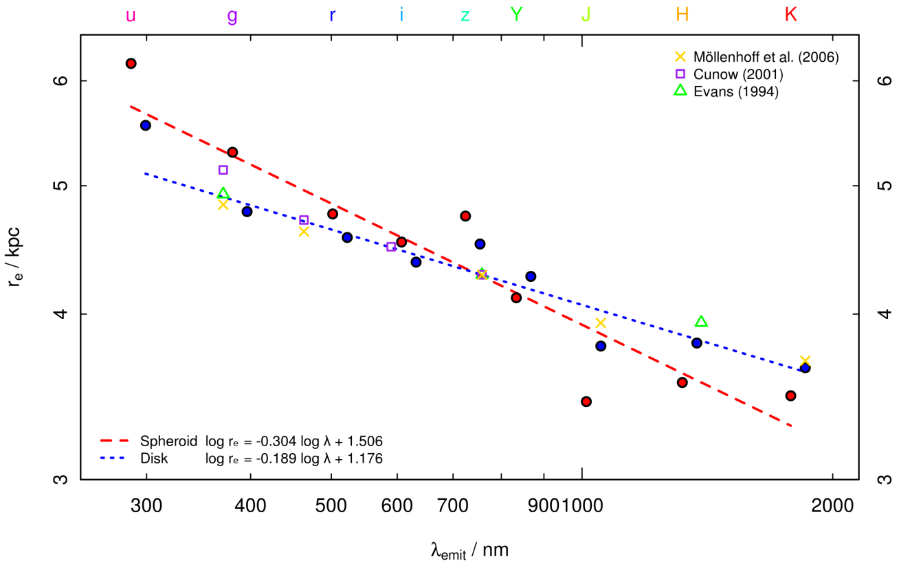
Figure 22. Recovered half-light radii in kpc as a function of rest-frame wavelength. Red and blue circles show the 3\sigma -clipped mean half-light radii for spheroid-dominated and disk-dominated galaxies respectively in each band, positioned at the median-redshift rest-frame wavelength for that population. Linear fits to these mean half-light radii are shown for both populations, the equations of which are inset into the figure. Owing to its lower quality imaging data, we exclude the u -band data in the calculation of these lines. Overlaid are data from several authors who predict an increase in the measured half-light radii in late-type systems due to the effects of dust. Further details are available in the text.
