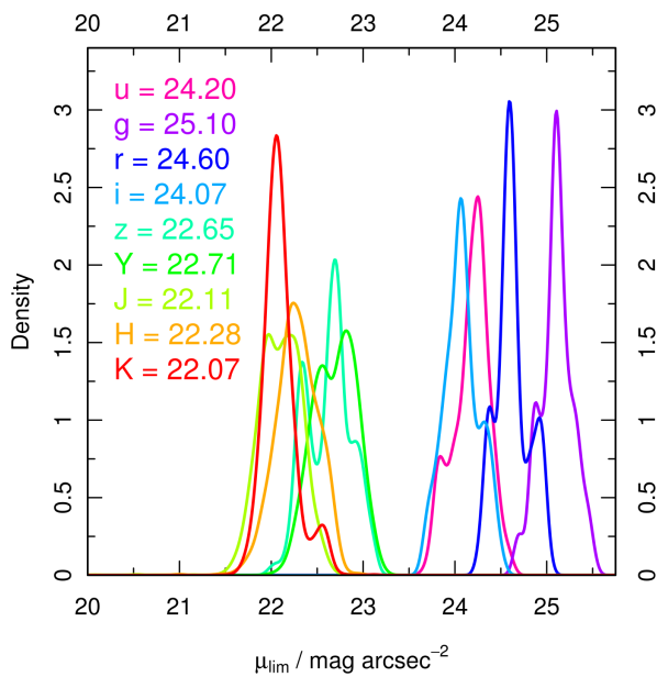
Figure 11. Apparent surface brightness limits for all galaxies within the SIGMA common coverage sample, with median surface brightness values for each band inset.
